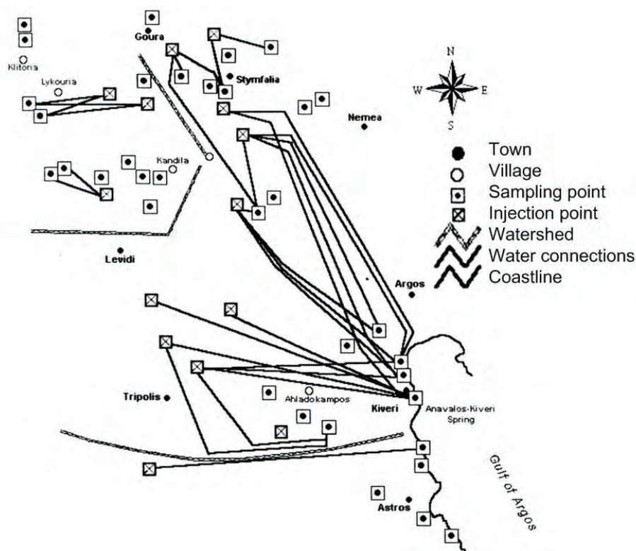
Fig. 19. Underground water connections of the Peloponnese, found by tracing experiments (Gospodarič & Leibung, 1986).
