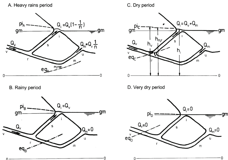
Fig. 7. Coastal spring with a siphon-like lower vein in a karst conduit flow aquifer, \pi_i - piezometric surface, eq - equilibrium plane. Four Flow: Salinity regimes (Breznik, 1989; 1998).
