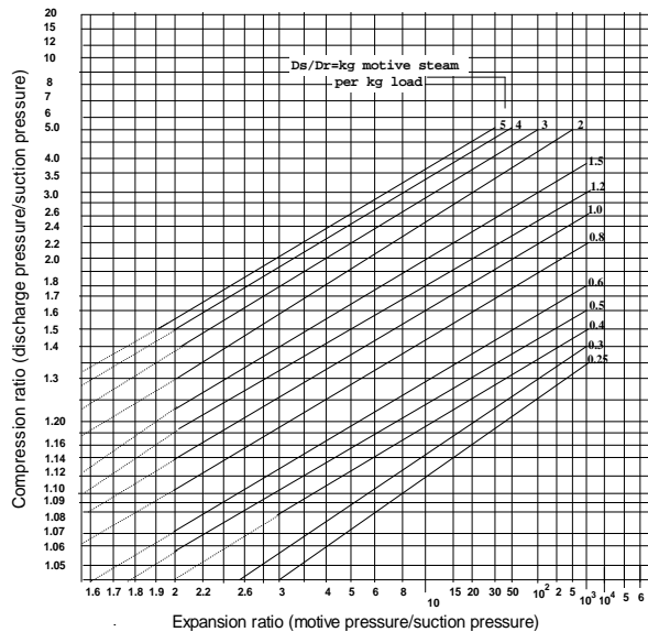
Fig. 3. Entrainment ratio for different compression and expansion ratios (Power, 1994)
