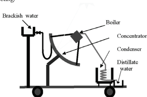
Fig. 15. Experimental device.
