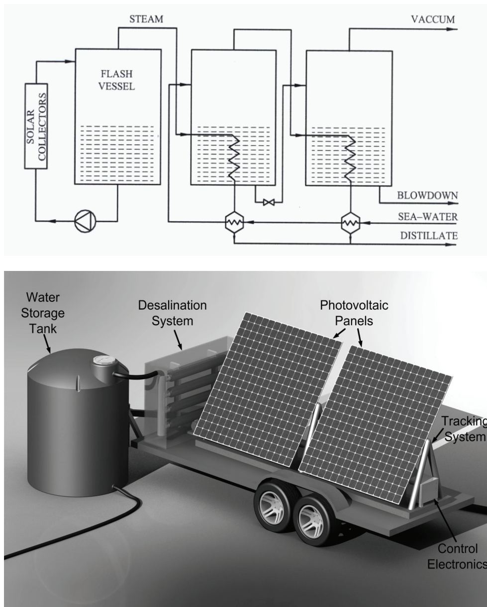
Fig. 9. a. (Top) Schematic of a multiple effect boiler (MEB) (Kalogirou (2005). 9b. (Bottom) A simple mobile solar powered reverse osmosis system (Dubowsky, 2010).
